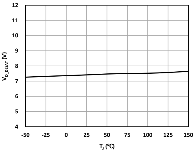
Figure 14. DESAT Threshold Voltage vs Temperature
