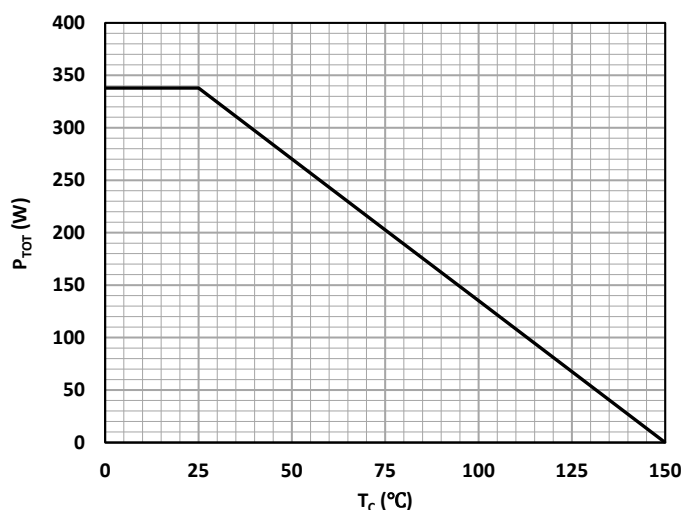
Figure 9. Power Dissipation
