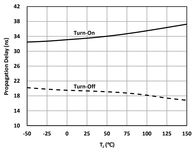
Figure 12. Turn-On/Off Propagation Delay vs Temperature
