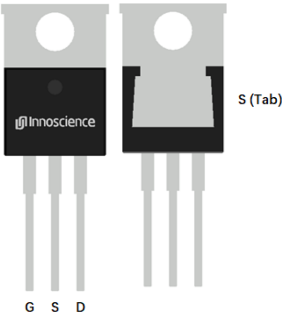
3-Lead TO220 Package – Top and Bottom View
