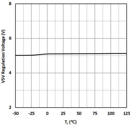
Fig. 14. V5V Regulation Voltage vs Temperature
