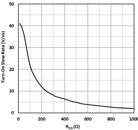
Fig. 17. Switch Slew Rate vs R DD Resistor
