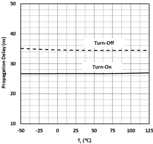
Fig. 16. Propagation Delay vs Temperature
