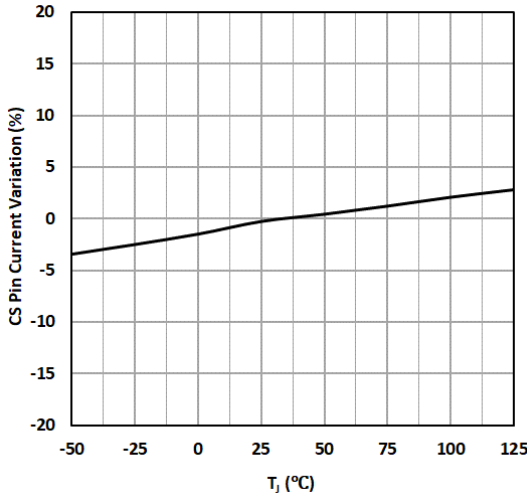
Fig. 18. CS Pin Current Variation vs Temperature
