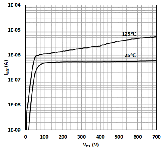
Fig. 4. Drain Leakage Current vs Drain Voltage
