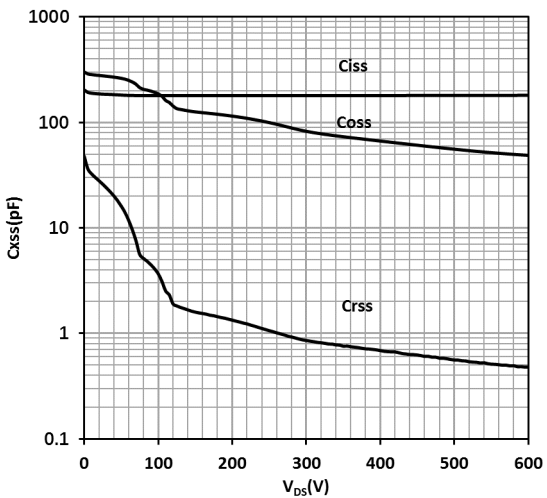
Figure 19 Typ. capacitances
