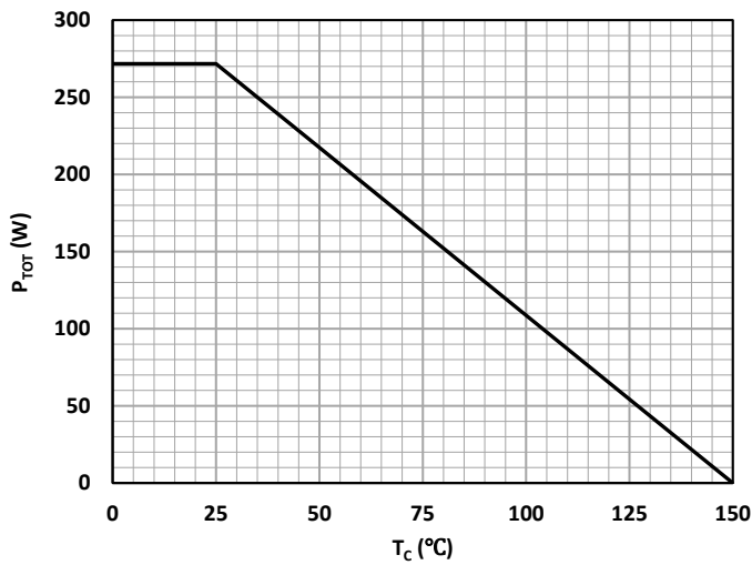
Figure 9. Power Dissipation
